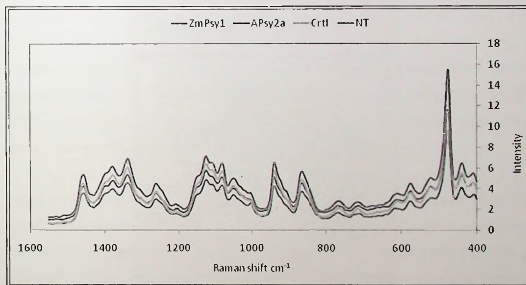
Figure 3.22 Close up of Raman spectra in the range 400\text{--}1500\text{ cm}^{-1} for rice seed. The Raman shifts observed show characteristic peaks for starch. No peaks corresponding to \beta -carotene were observed in transgenic rice seed.
