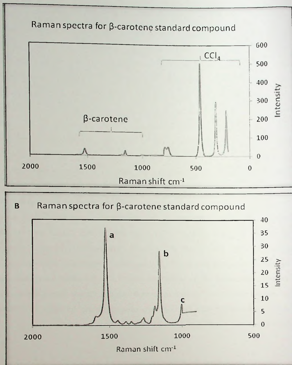
Figure 3.2 Raman spectra for \beta -carotene standard compound. Graph A shows the spectrum for \beta -carotene peaks in the range 1000 - 1550 \text{cm}^{-1} and peaks of carbon tetrachloride in the range 200 - 800 \text{cm}^{-1} Raman shift. Graph B shows a close-up of the Raman spectra for \beta -carotene with peaks for C=C at 1523 \text{cm}^{-1} (a), C-C at 1156 \text{cm}^{-1} (b) and \text{CH}_3 (c) at 1003 \text{cm}^{-1} Raman shift
