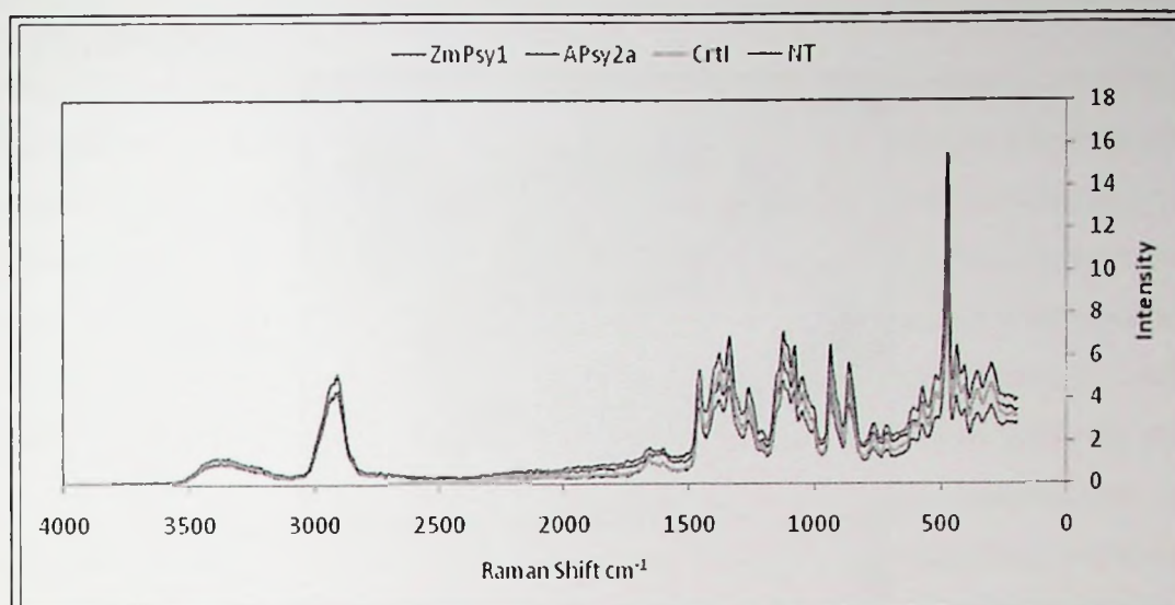
Figure 3.21 Full Raman spectra for representative rice seed for in-situ detection of pVA carotenoids
