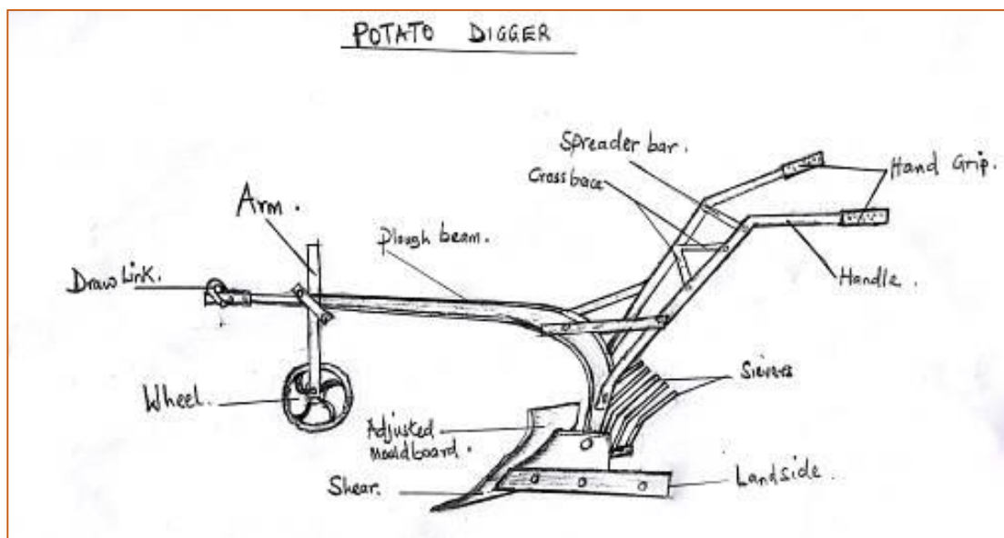
Figure 2: Sketch of Ox-potato lifter showing the different components
